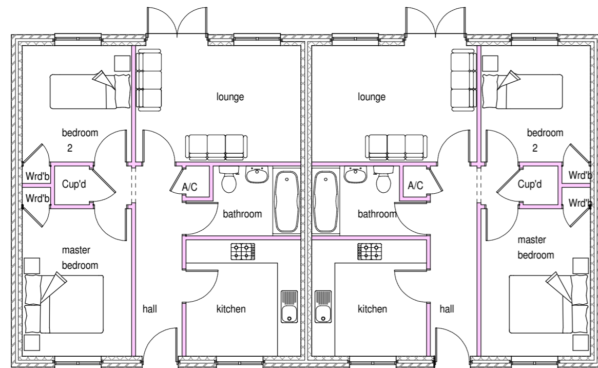
1 GROUND FLOOR PLAN 1:100
