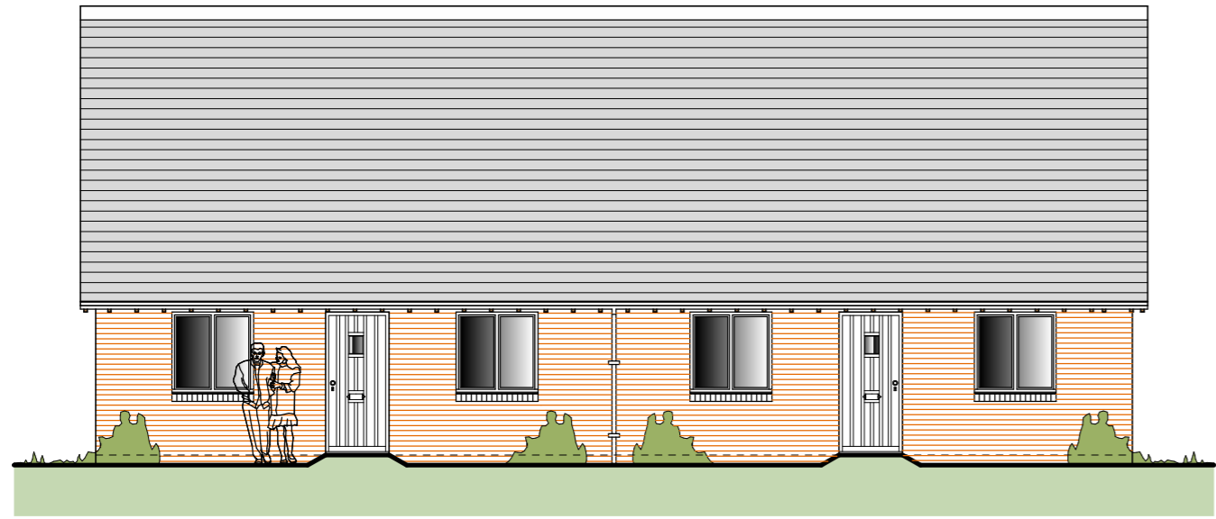
2 FRONT ELEVATION 1:100
